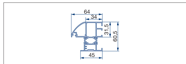
Roundstyle frame
