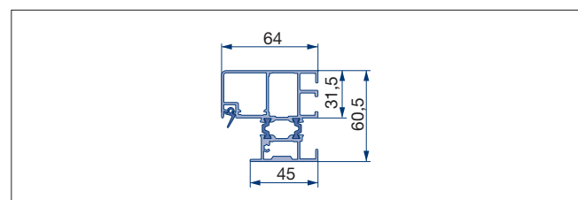
Quadrangular frame
