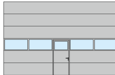
SPU F42, SPU 67 Thermo Aluminium glazing frames Wicket door in the centre
