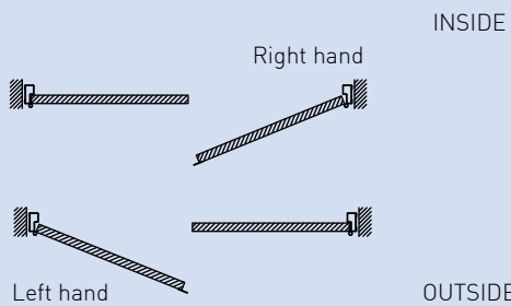
Double blade outward opening
