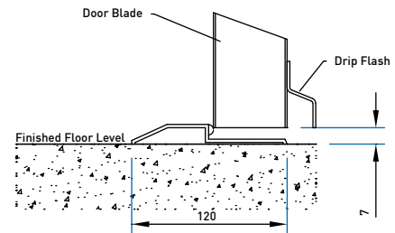
Low Profile Aluminium Threshold with Drip Flash
