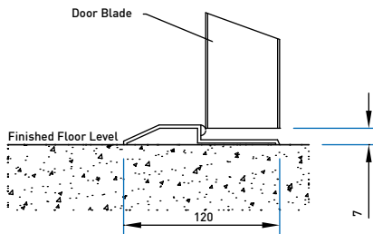
Low Profile Aluminium Threshold
