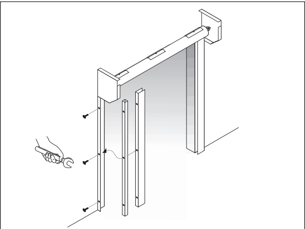
7 Attach the channels and the 30x30 box section to the angles if applicable.
