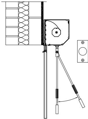
Rigid Eye Joint
