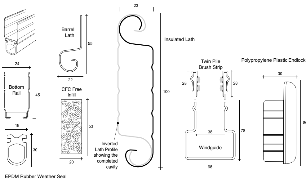
EPDM Rubber Weather Seal
