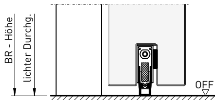
Retractable bottom seal
