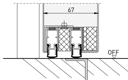
Double retractable bottom sea (for highly sound-insulated doors)
