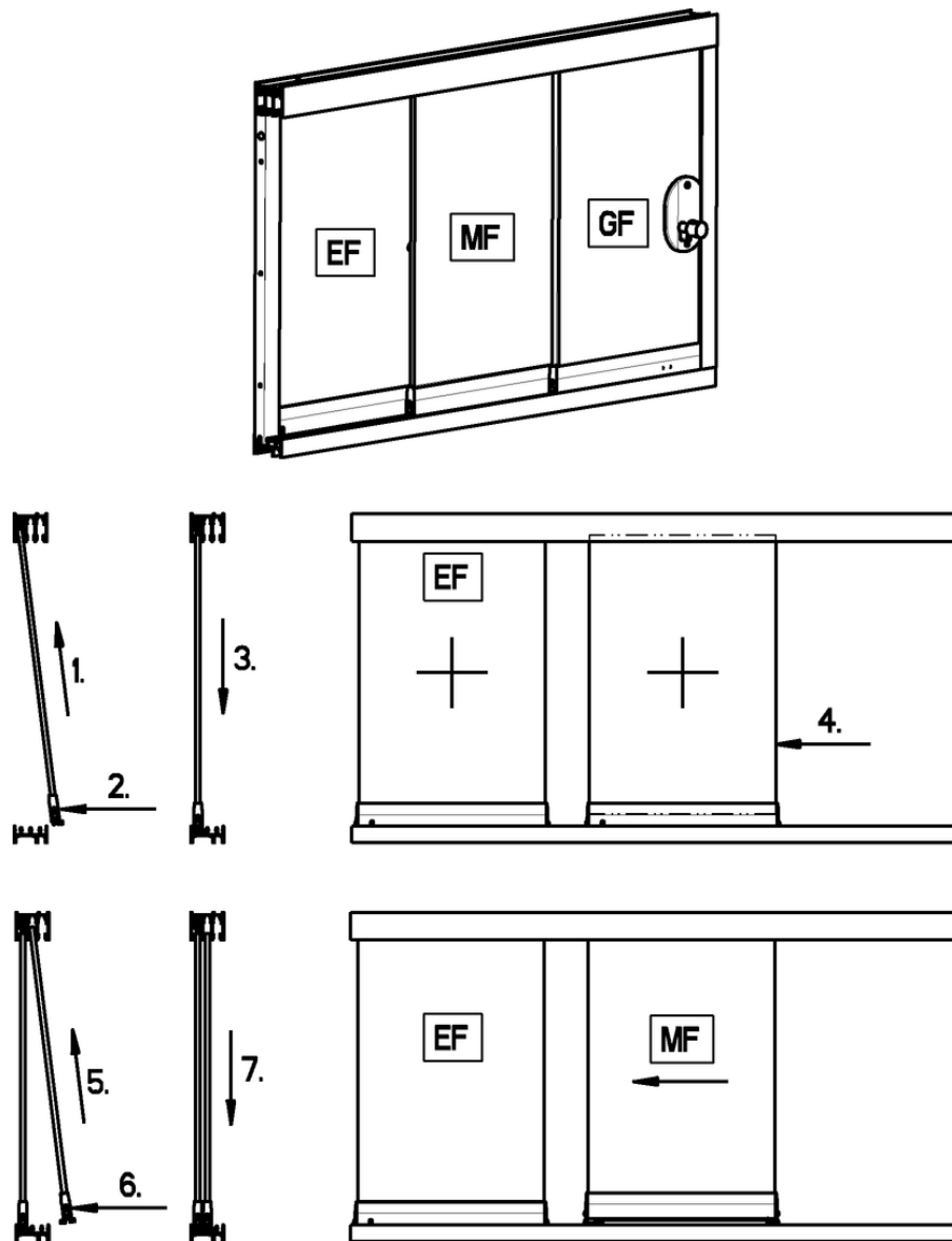
Figure 50: Inserting the leafs on lockcase with hung bolt versions
