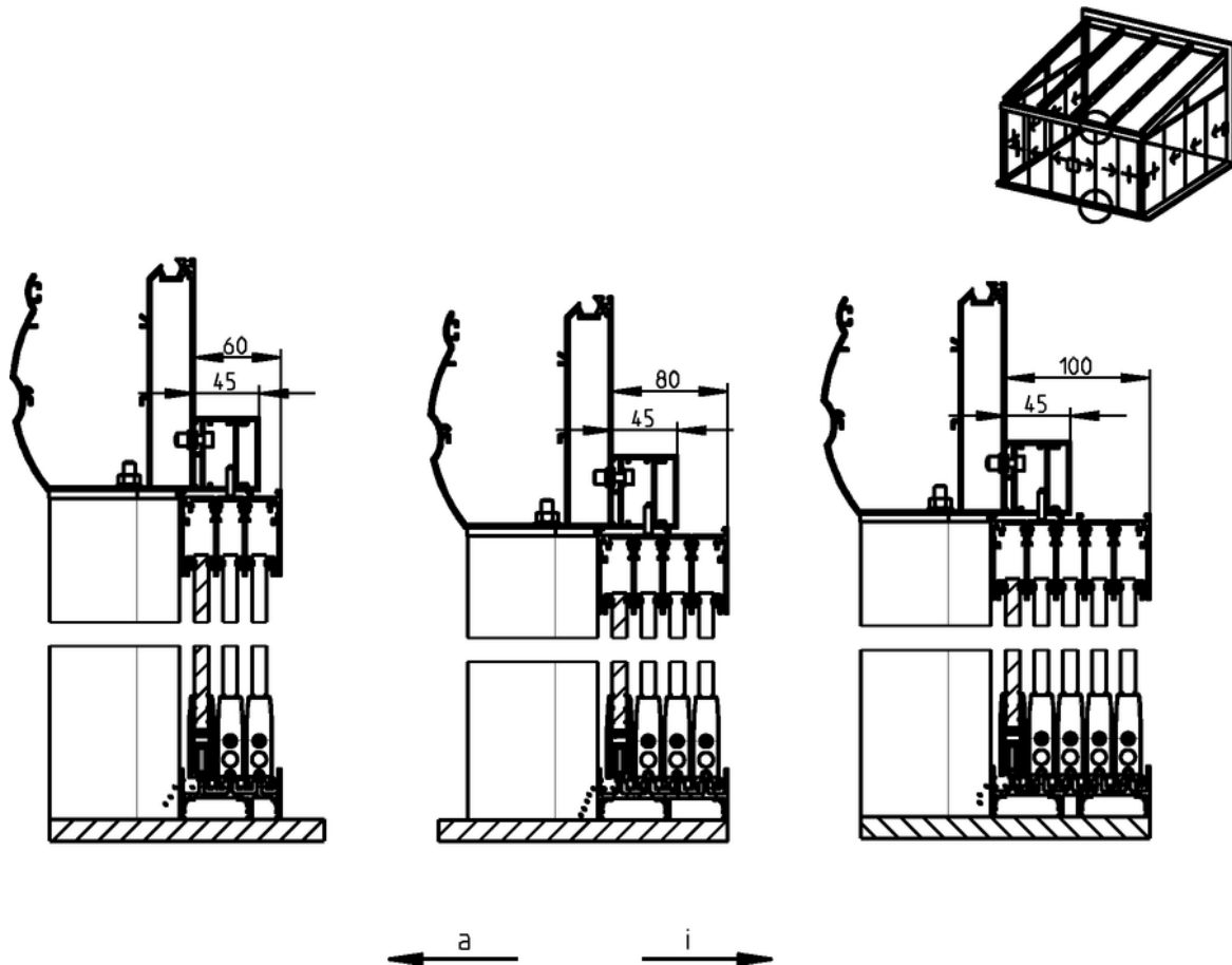
Figure 43: Assembly of the guide profiles behind the post, 3 to 5 tracks
