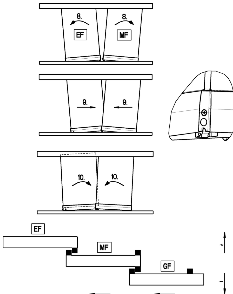
Figure 51: Attaching leafs using the additional actuators
