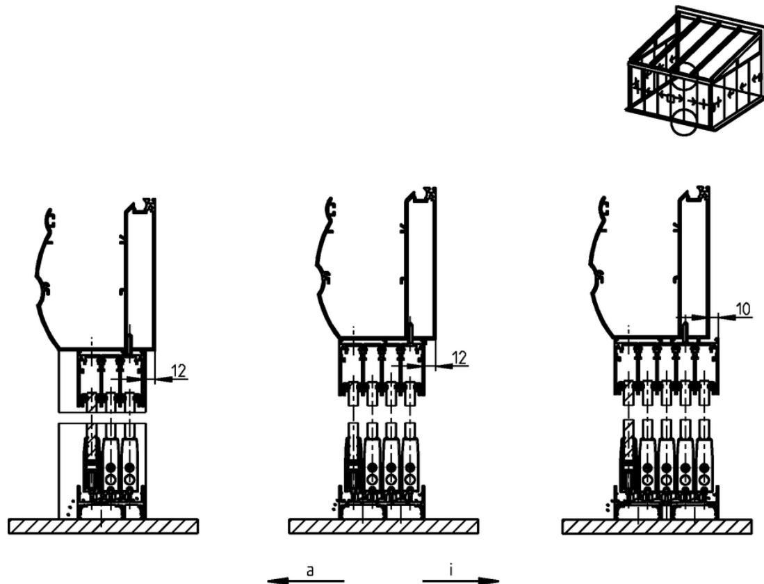
Figure 11: Assembly of the 3- to 5-track guide profiles below the gutter
