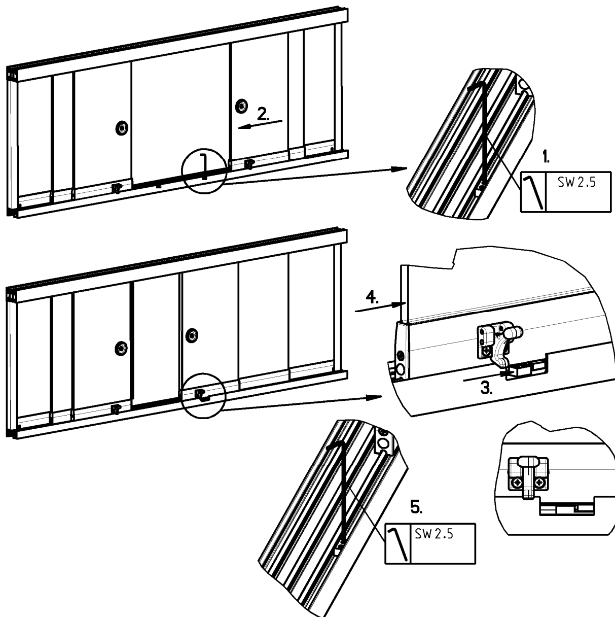
Figure 34: Adjusting sets of leafs on lockplate versions
