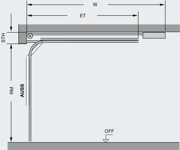
Sectional door with track application L
