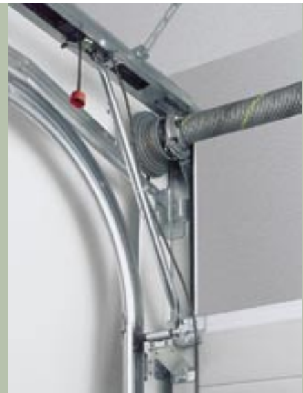
Fitting for Hörmann high-lift sectional doors
