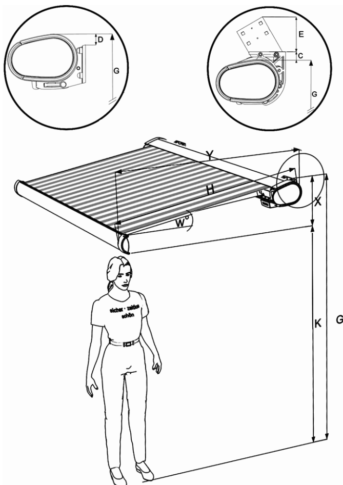
BS-Ceiling fixture 5 - 35° C = 30 mm
