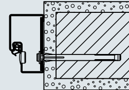
Block frame Fitting to brickwork Plug-and-screw fitting
