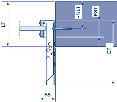
Space requirements of support bracket
