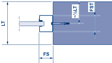
Space requirements of side guide FS60 x 75
