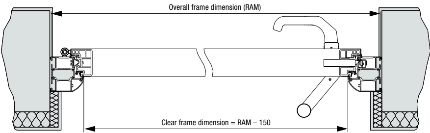
Horizontal view of door, Thermo65
