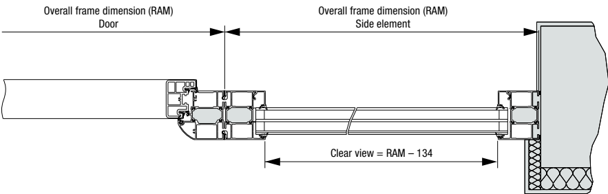
Frame variants, Thermo65
