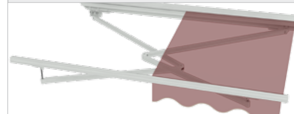
arms cross above one another during extension
