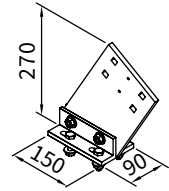
eaves fixture bracket 270 mm
