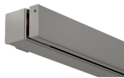
5 hidden gutter in the front profile with water drainage holes to the side
