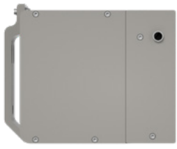
3 arm bearer with tilt device technology, integrated windlock mechanism
