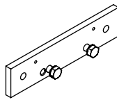
supplementary flat plate eaves fixture 260 x 60 x 12 mm
