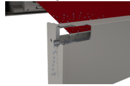
5 hidden gutter in the front profile with water drainage holes to the side
