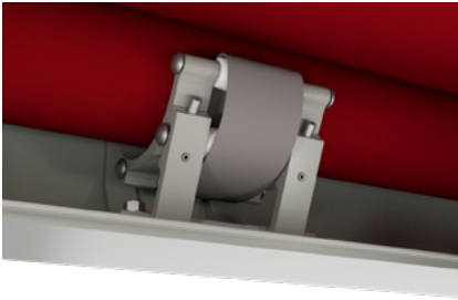
6 rolltex bearing for the roller tube, used in larger awning widths
