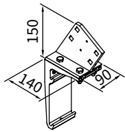
eaves fixture bracket 90 mm
