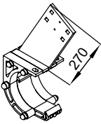
eaves fixture bracket 270 mm 5°–35°
