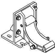
bottom fixture 5°-35°
