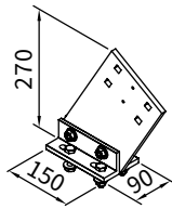
eaves fixture bracket height of flat plate: 270 mm
