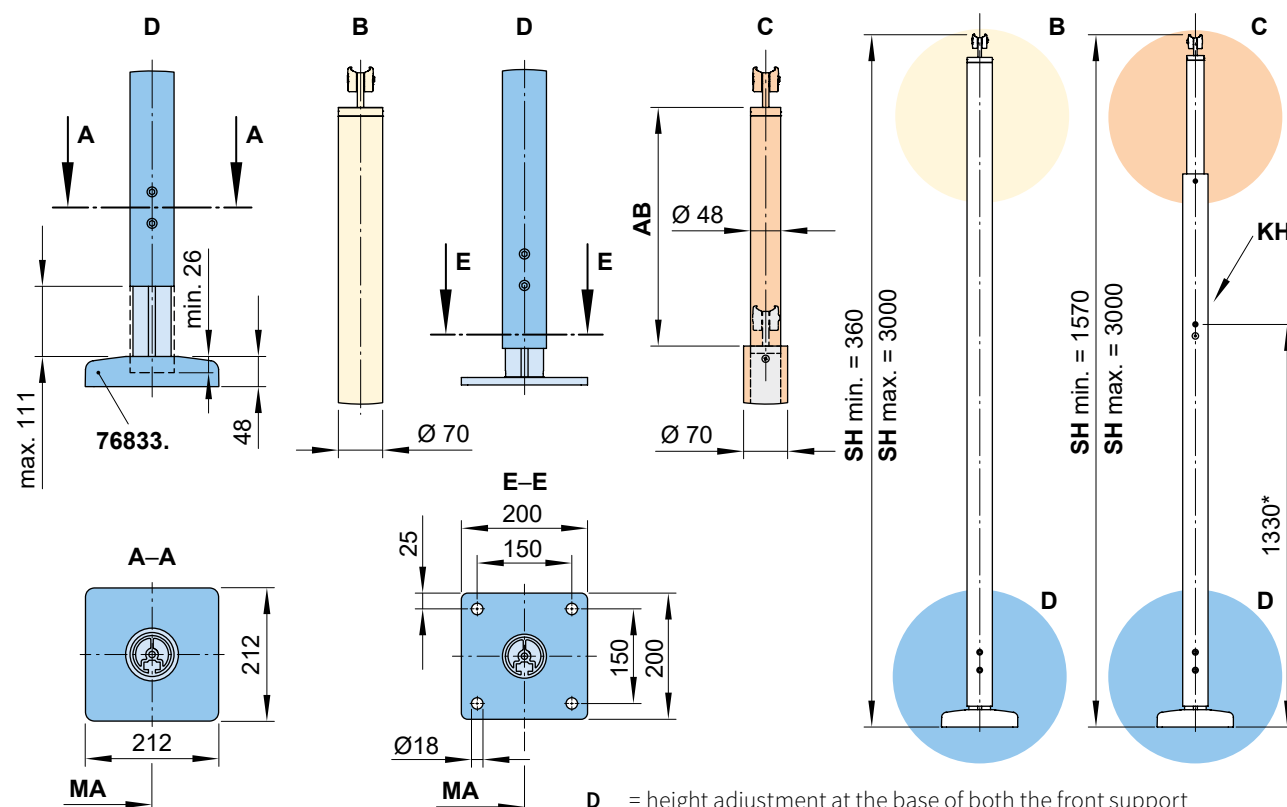
Round support post with footplate (not adjustable/adjustable)
